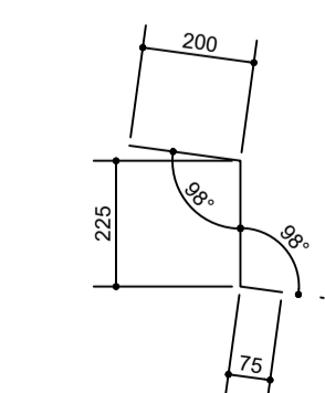
Z1 Flashing 4.5m lengths - 1.6mm gauge 15no. lengths
